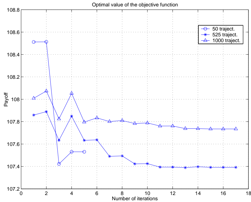
Figure 2: Objective function history. Different number of trajectories
