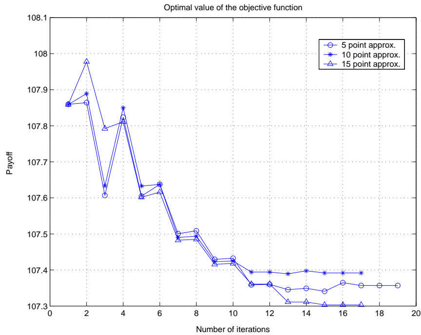
Figure 8: Objective function history. Different problem sizes
